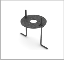
Ordering Code: 9-2014-00 Anchor Bolt Kit for Bollard
